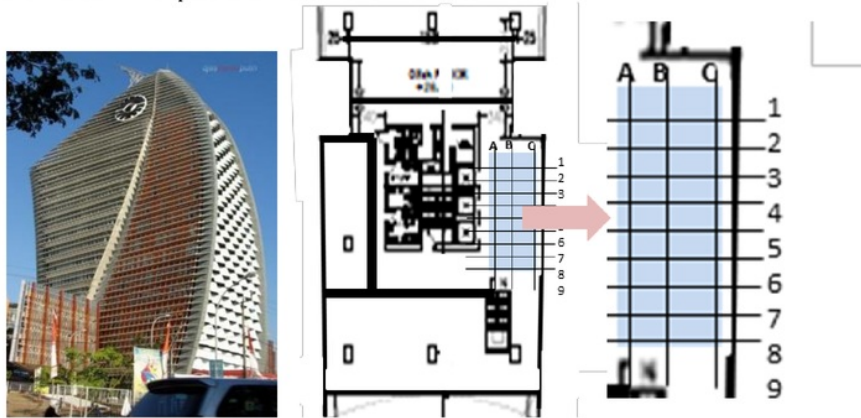
Figure 6. Placement of measurement points in the lobby area (8 th floor)
